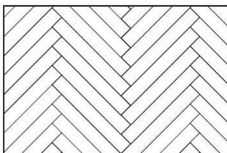
Herring bone installation 45°
